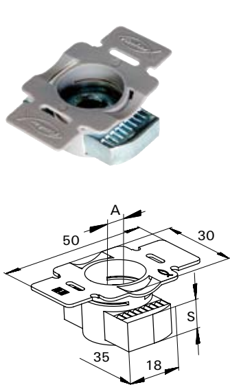
FCN Clix P
